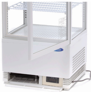
Digital temperature controller on frontside
